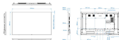
Philips 65BDL3552T Version 1.1 Release Date: 2019/12/20
